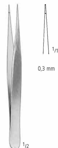
WISE AB 534/13 13,5 cm/5 1 / 4 "
