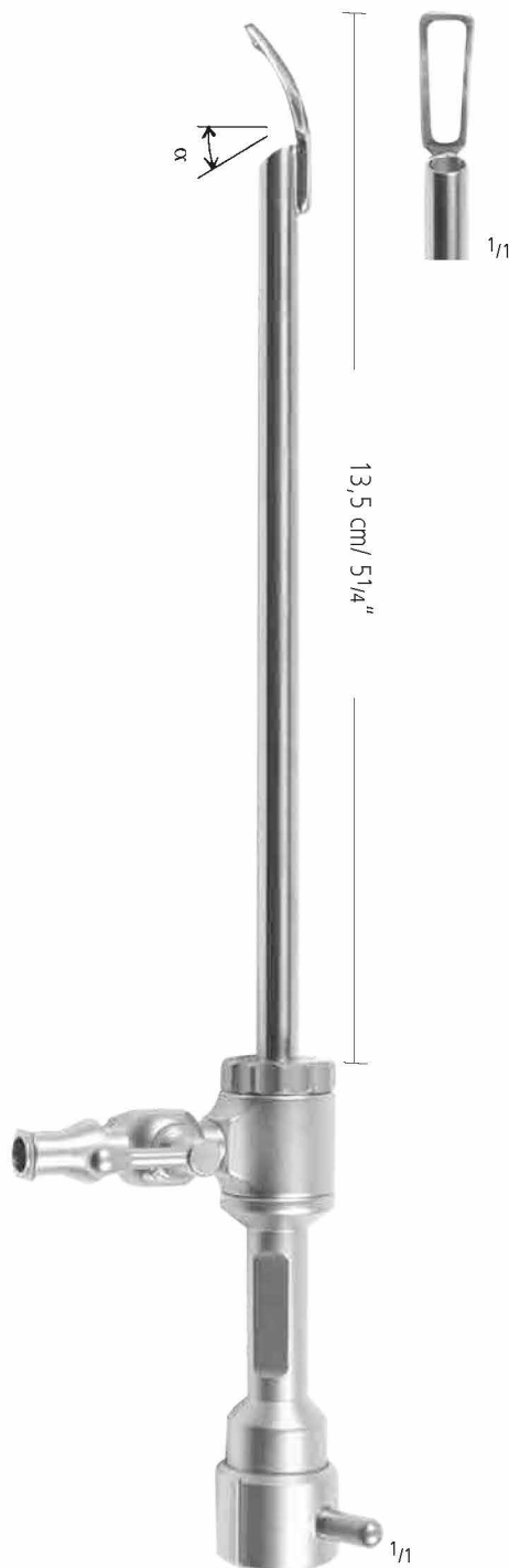
OPTICAL DISSECTOR FOR ENDOSCOPES AK 456/01 175 mm, Ø 4,0 mm \alpha = 30^\circ
