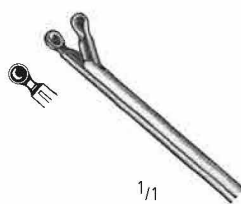
HARTMANN KM 238/20 = 2,0 mm KM 238/25 = 2,5 mm KM 238/30 = 3,0 mm
